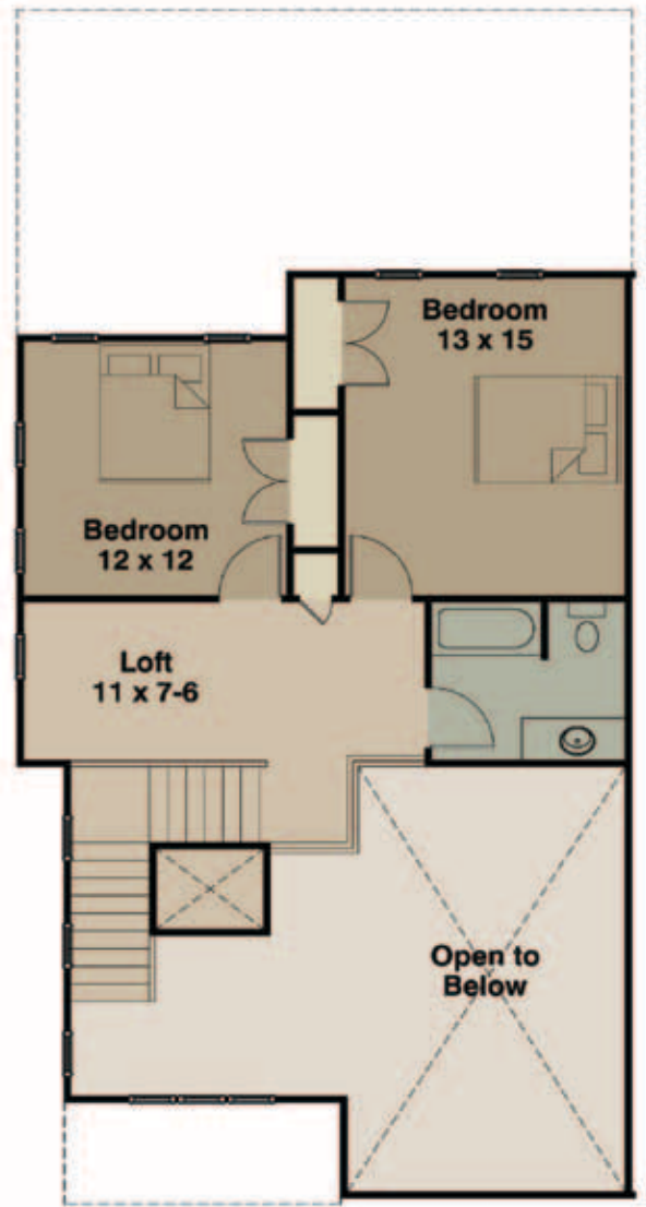
SECOND FLOOR
